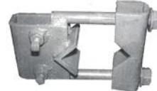
For 3-1/2" to 4" Diamond Bar
